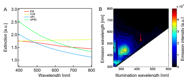
Figure 2. (A) Extinction spectra of aqueous CB suspensions. (B) Two-dimensional excitation–emission plot of uPPL particles in water under single photon excitation with a false color map based on the emission intensity in arbitrary units. The red arrow points toward the Raman line of water.
